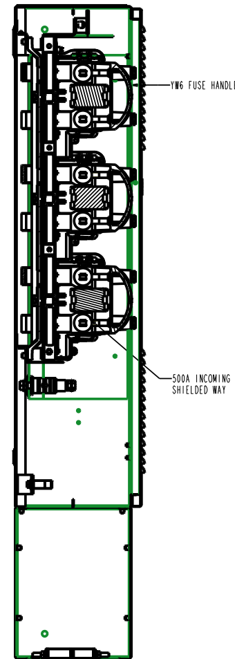
SECTION A-A SHOWING 500A INCOMING SHIELDED FUSEWAY
