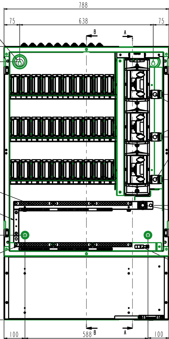
FRONT VIEW WITH DOOR AND INCOMING CABLE SCREEN REMOVED
